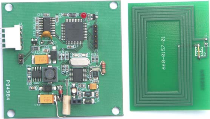
Reader PCB Reader Antenna
