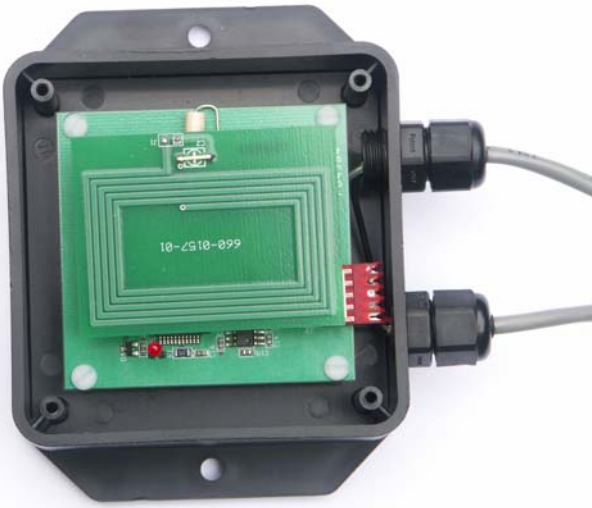
Reader Mounted in Housing (lid not shown)
